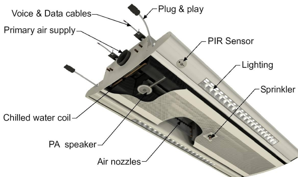
Fig 1. Typical Active Type Multi-Service Chilled Beam (MSCB).
