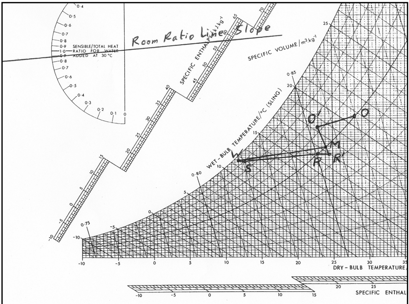
Figure 1 – Psychrometric Diagram of Fan Coil Unit, Summer Cooling Cycle
